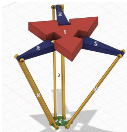
Figura 1. Robot delta [4].
